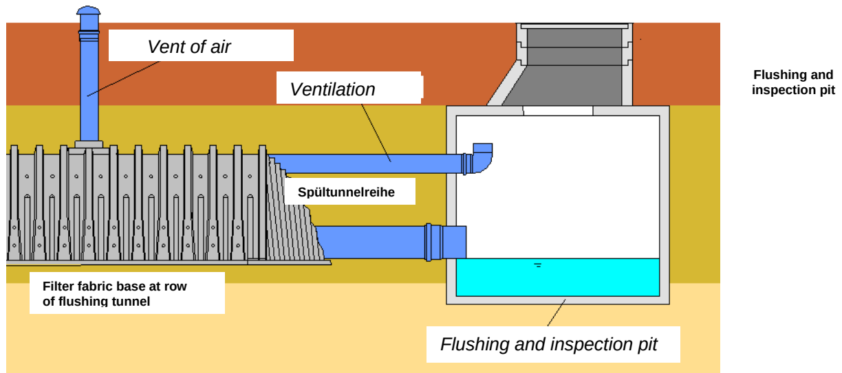
Fig. 12: Example for venting possibility
