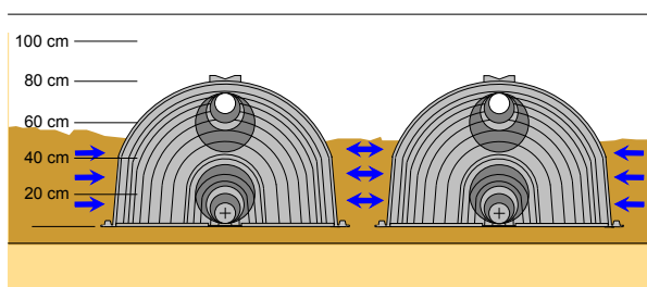
Fig. 13: not permitted, one sided backfilling
