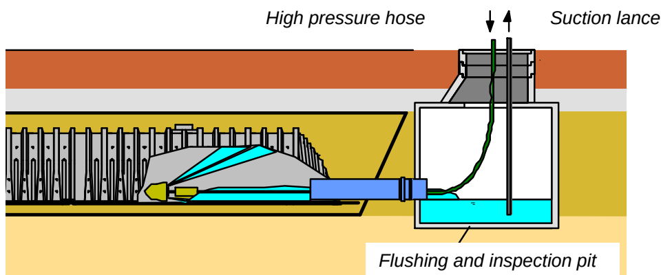
Fig. 8: Cleaning and slime removal via flushing and inspection pit
