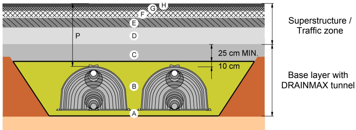
Fig. 18: Example of base layer / superstructure with bituminous cover in accordance with RStO classification V, Line 3.1 1
